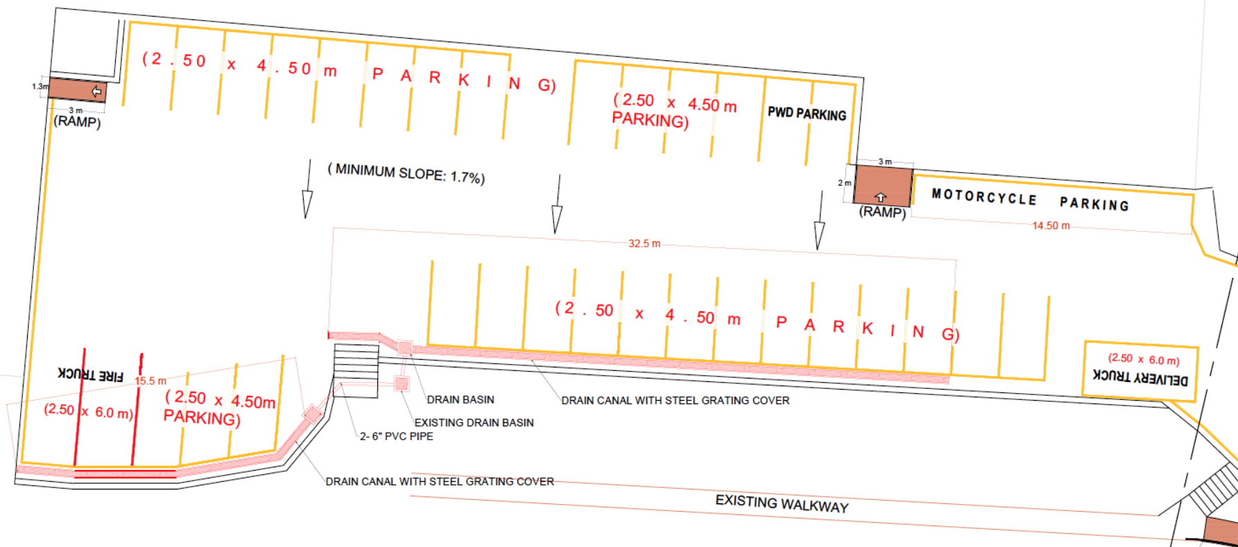
MAIN PARKING PLAN (NTS)
