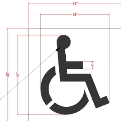
PWD MARKING DETAILS NTS
