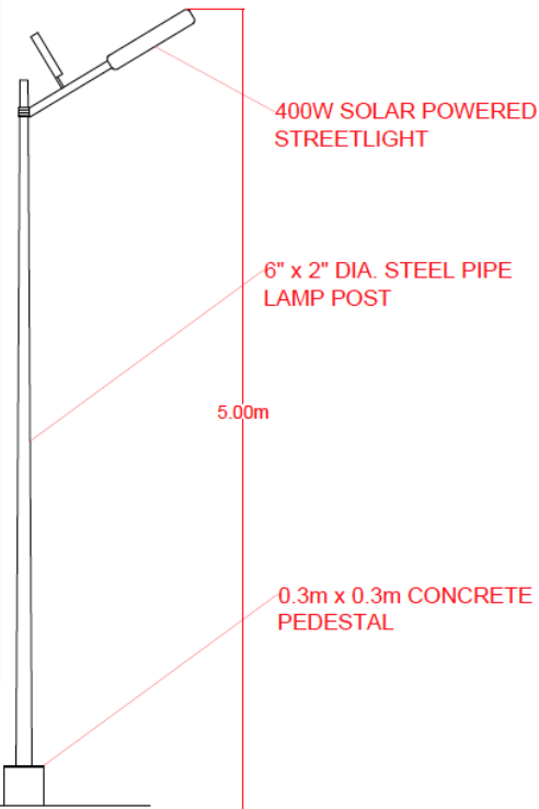
STREET LIGHT ELEVATION
